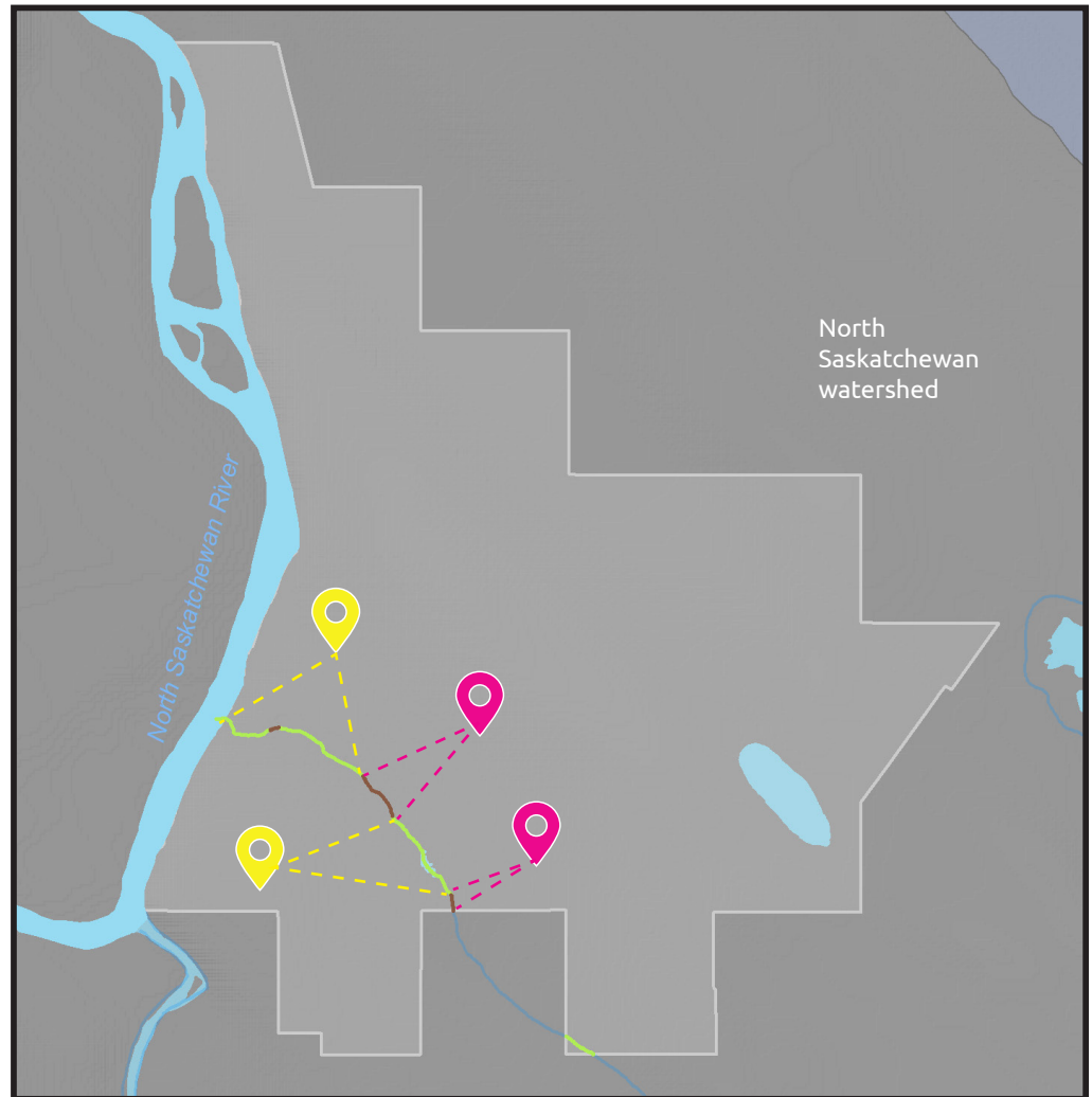
Map 4: The top Conservation and Restoration Priorities recommended for the municipality. Recommendations are based on the top results from the Prioritization assessment shown in Map 3. To view more data, please see the attached Appendix .
